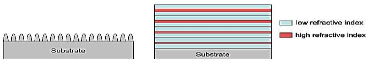
Figure 6: Comparison between a moth-eye structured surface (left) and an antireflective coating(right). Both methods reduce the reflection efficiently.
