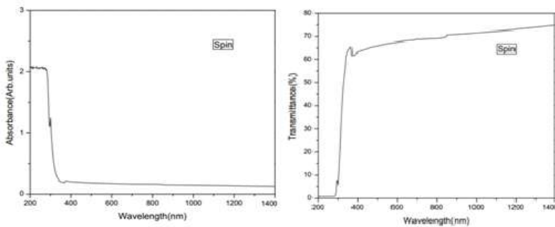
Fig 3 The Absorbance and Transmittance spectra of as deposited ZnS thin film
