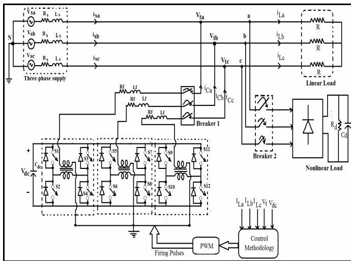
Fig.1. Schematic diagram of VSI-based DSTATCOM
