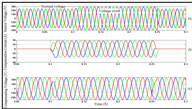
Fig.10 Voltage swells under nonlinear load with PI control scheme
