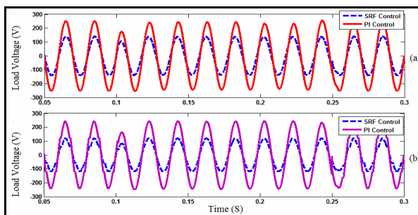
Fig.12. Comparison of load voltage under SRF and PI control techniques (a) linear load and (b) Nonlinear
