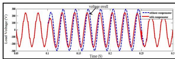
Fig.11. Load voltage with and without compensator under nonlinear load with PI controller
