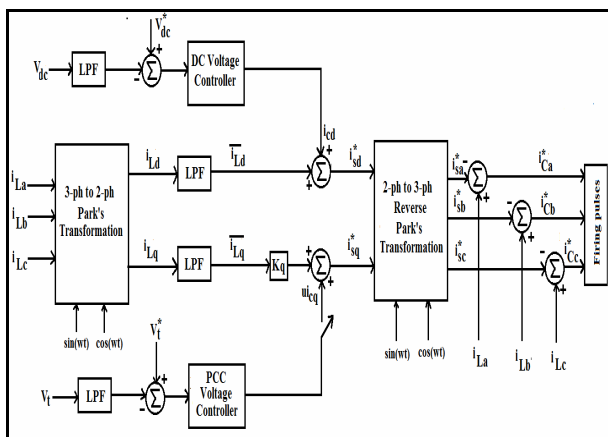
Fig. 2. Block diagram of SRF controller
