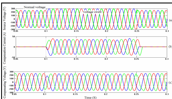
Fig.8 Voltage swells under linear load with PI control scheme
