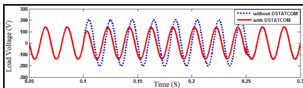
Fig. 5. Load voltage with and without DSTATCOM by SRF controller
