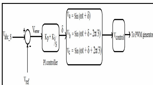
Fig.3. PI Controller
