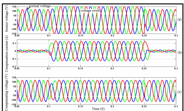
Fig. 6. Voltage swell under nonlinear load with SRF theory
