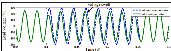
Fig.9. Load voltage with and without compensator under linear load with PI controller
