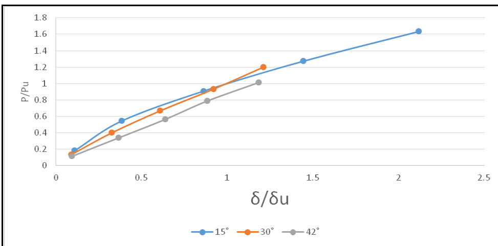
Figure 8: P/P_u Vs \Delta/\Delta_u for 4x4 Pile-4d Spacing
