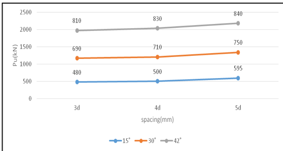
Figure 4: Ultimate Load Vs Spacing Between Piles for 3x3 Piles
