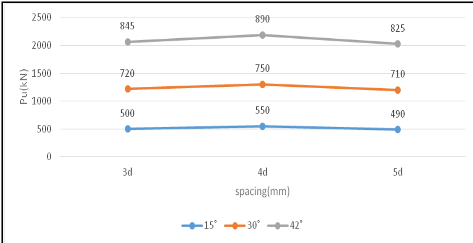
Figure 5: Ultimate Load Vs Spacing Between Piles for 4x4 Piles
