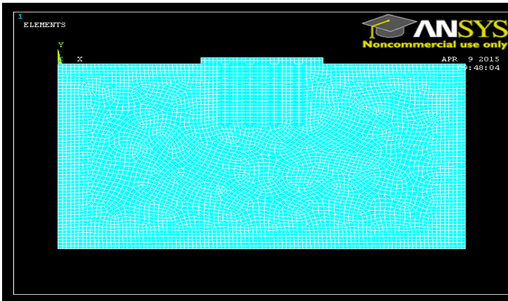
Figure 2: Meshed Model of 4x4 Pile Group
