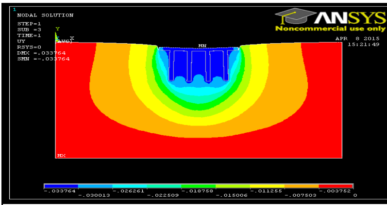
Figure 3: Contour Diagram of 4x4 Pile Group
