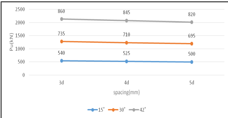
Figure 6: Ultimate Load Vs Spacing Between Piles for 5x5 Piles
