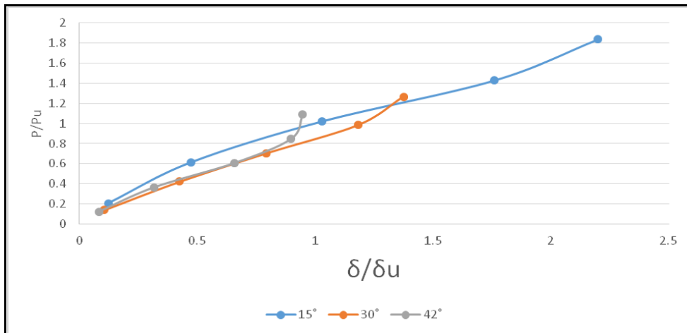
Figure 9: P/P_u Vs \Delta/\Delta_u for 4x4 Pile-5d Spacing
