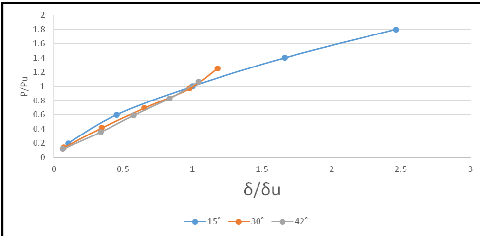
Figure 7: P/P_u Vs \Delta/\Delta_u For 4x4 Pile-3d Spacing
